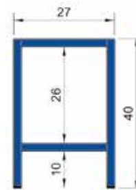
Floor rack for boots
